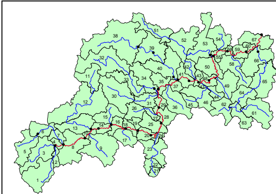
Fig 2.31. Representation of Ipswich watershed in HSPF illustrating 67 sub-basins (black lines and numbers), main stem of Ipswich River (red line) and major tributaries (blue lines).
