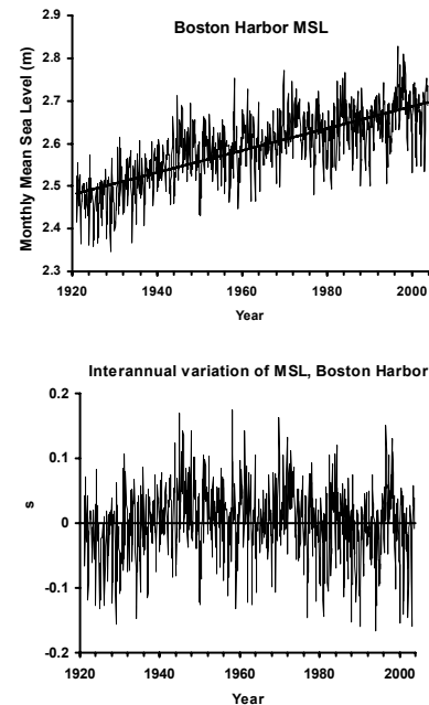
Fig 2.4. Sea level rise is a global issue. Over the past 80 years at PIE, it has been increasing at a rate of 2.65 \text{ mm yr}^{-1} as recorded at the Boston NOAA station. Superimposed on the long-term trend is substantial monthly and annual variability. Short-term changes in mean sea level on the order of 20-30 cm can mean the difference between whether the marsh floods or not.
