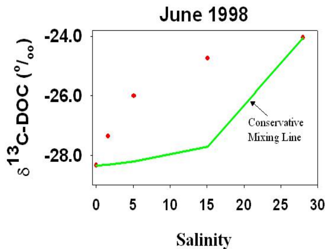
Fig. 2.20. Delta ^{13}\text{C-DOC} in the Parker River, June 1998 shown by circles. Also shown is the conservative mixing line that indicates the values if only mixing of the freshwater and seawater occurred. Methods are given in Raymond and Hopkinson (2003).
