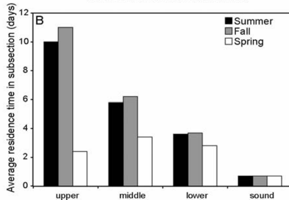
Fig 2.19. Average residence time of water in each subsection on summer, fall, and spring sampling dates (from Crump et al. (in press)).
