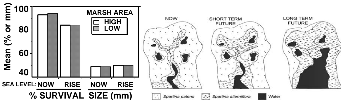
Fig 2.28. Preliminary results from a spatially explicit, individually-based simulation model indicate that in all marsh configurations rising sea level will decrease survivorship due to increased exposure to predators, but will have little effect on growth. The model simulated hourly movement, mortality, and growth of individual mummichogs (Haas and Deegan, in prep.) on a 50 m x 50 m spatial grid of 1-m 2 cells (using a digital orthoquad of Sweeney Creek as the base and projected marsh area change) for 14 days for a cohort of 500 mummichogs. Each fish was assigned an initial length ( 30 \pm 2.5 mm), baseline growth ( 1 \pm 0.25 mm d -1 ) and mortality ( 0.0003\% \text{ h}^{-1} ) from a normal distribution. To simulate fish movement from creeks onto and across the marsh, fish consider the cells within 1m, then within 2 m, of their current position and moved to the shallowest, yet still inundated, cell in their neighborhood. Predation and growth were then calculated hourly depending on fish position and habitat (predation in open water was 1.75 and in marsh 0.5 times baseline; growth in marsh was 1.25 times baseline).
