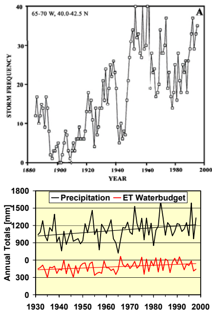
Fig 2.3. Storminess has increased with increasing latitude in the past century, with it tripling at PIE (Hayden and Hayden 2003). We have evidence that both precipitation and evapotranspiration have increased over the past 70 years in the Ipswich River watershed (Claessens et al. submitted). The relatively greater increase in ET has resulted in a net decrease in the river runoff coefficient. Changes to the hydrologic cycle are occurring worldwide (Peterson et al. 2003).
