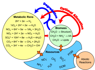
Fig 2.40 Conceptualization of the metabolic biogeochemistry model. Half reactions lead to production of protein (and other building block constituents), which is then allocated to reactions governed by an optimization function. Abiotic reaction can also be incorporated with standard kinetics.
