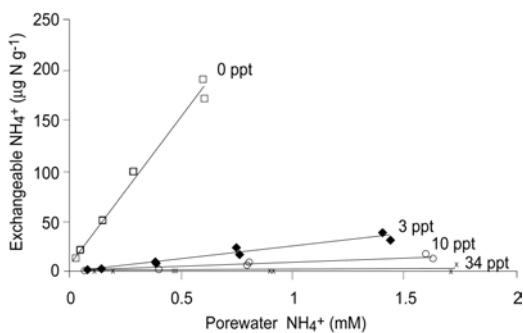
Fig 2.23. Changes in the ratio of adsorbed (exchangeable) NH 4 + and dissolved NH 4 + in the porewater with salinity in sediments from the upper Parker River Estuary. At 0 PSU, approximately 68% of the NH 4 + in sediments is adsorbed onto particles while less than 32% is dissolved and free to diffuse into overlying waters. At high salinity nearly all of the NH 4 + is free. This leads to a large efflux of NH 4 + from sediments in mid-summer (Weston in prep, Hopkinson et al. 1999).
