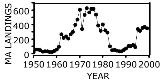
Fig 2.27. In the Rowley River (1999) about 60% of striped bass diet is based on species that use salt marshes such as mummichog, A. silverside and Crangon (Ferry 2003). Striped bass population size in MA is increasing suggesting that their predatory impact is increasing (Div. Marine Fisheries data).
