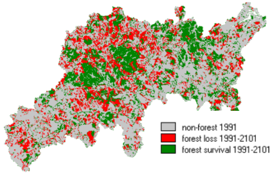
Fig 2.8. Land use change models have been developed using historical land use data to predict deforestation in the Ipswich watershed over the next century (Schneider and Pontius 2001). Predicted changes have been linked with biogeochemical models to model future changes in water and nutrient exports. We will develop maps of forest and residential age to understand contemporary variability in nutrient export.
