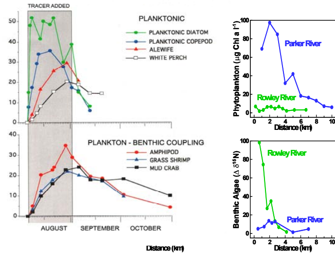
Fig 2.6. Evidence from a whole system ^{15}\text{N} addition experiment for both planktonic and benthic foodweb links between bloom-forming phytoplankton and higher trophic levels. Graph shows the isotopic enrichment of water column and benthic organisms in the upper Parker River during and after isotope addition. The planktonic copepod and benthic amphipod became equally enriched relative to the bloom-forming diatom. Enrichment patterns show that two fish, alewife and juvenile white perch, feed in the water column on planktonic copepods and that larger white perch become increasingly benthivorous (Hughes et al. 2000). Graphs to the right illustrate the importance of water residence time: when water residence time is long, phytoplankton are the principal primary producers (top right), while when residence time is short benthic algae are the principal autotrophs (Tobias et al. 2003).
