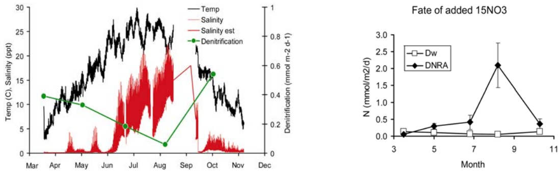
Fig 2.22. a) Temperature, salinity and rates of coupled nitrification and denitrification over the season in the Upper Parker River Estuary. Salinity increases over the summer as runoff decreases but also shows changes corresponding to spring neap and daily changes in tide height. Coupled nitrification/denitrification shows an inverse trend with temperature and reaches minimal rates during late summer when salinity is highest. b) The fate of added 15 N nitrate added to the sediments from the same site as above. In spring direct denitrification (Dw) exceeds dissimilatory nitrate reduction to ammonium (DNRA). DNRA peaks in late summer, as Dw and coupled nitrification/denitrification (Fig 4-1a above) reaches minimal values.
