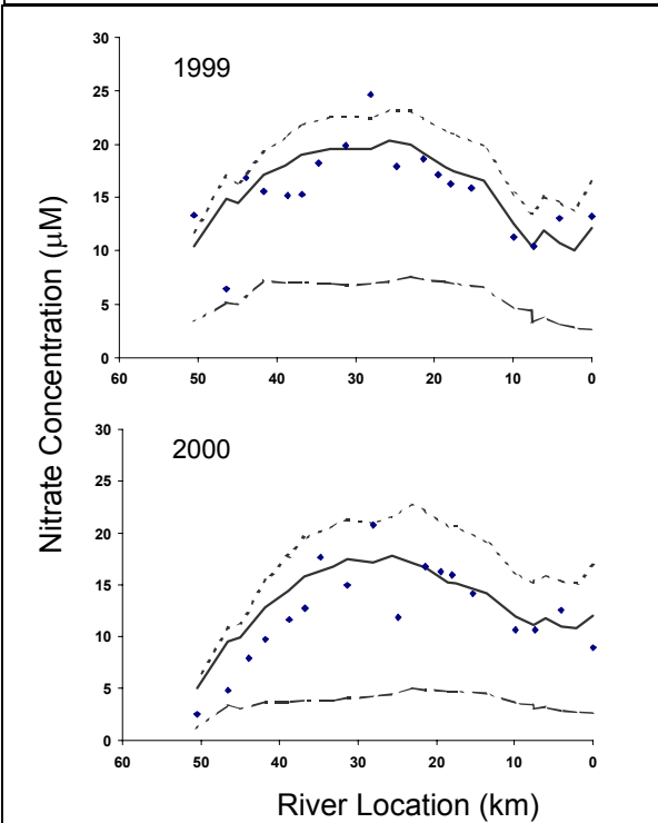
Fig 2.33. Nitrate concentrations along the main stem of the Ipswich River in 1999 (top) and 2000 (bottom). Annually averaged monthly observations (diamond symbols) compared to simulated values under current land-use conditions (solid line), 44% of current forests urbanized (short dash line), and prior to watershed colonization (long dash line).
