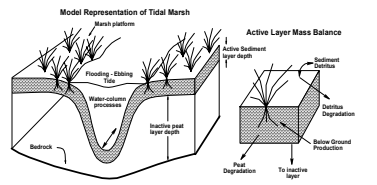
Fig 2.39 Marsh accretion and loss model. Marsh loss or accretion is determined by sediment loading and below ground production.
