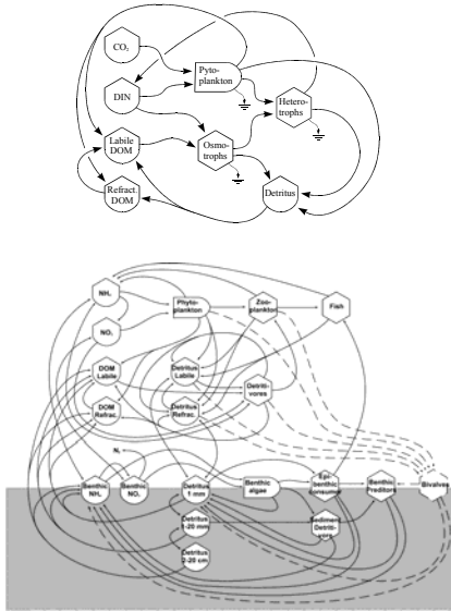
Fig 2.37. Example of simple (top) and complex (bottom) estuarine biogeochemistry models.
