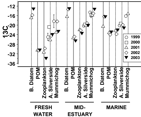
Fig 2.26. The different zones of influence are reflected in the overall more enriched \delta^{13}\text{C} values in the marine site compared to the riverine site. Isotopic variation within and among key functional groups is more variable in riverine influenced sites compared to marine influenced sites. Only 5 of the 10 functional groups sampled are plotted.
