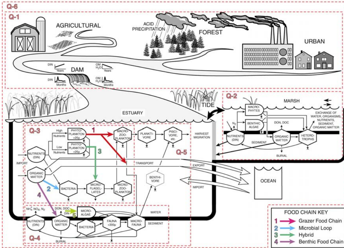
Fig 2.5. Conceptual model illustrating the collective integration (Q-6) of the biological and physical transformations of organic matter and inorganic nitrogen derived from watersheds (Q-1) and marshes (Q-2) and processed by organisms of the marsh (Q-2), estuarine water column (Q-3, Q-5) and benthos (Q-4). “Q”s and associated boxes refer to programmatic area covered by each of the Research Questions.
