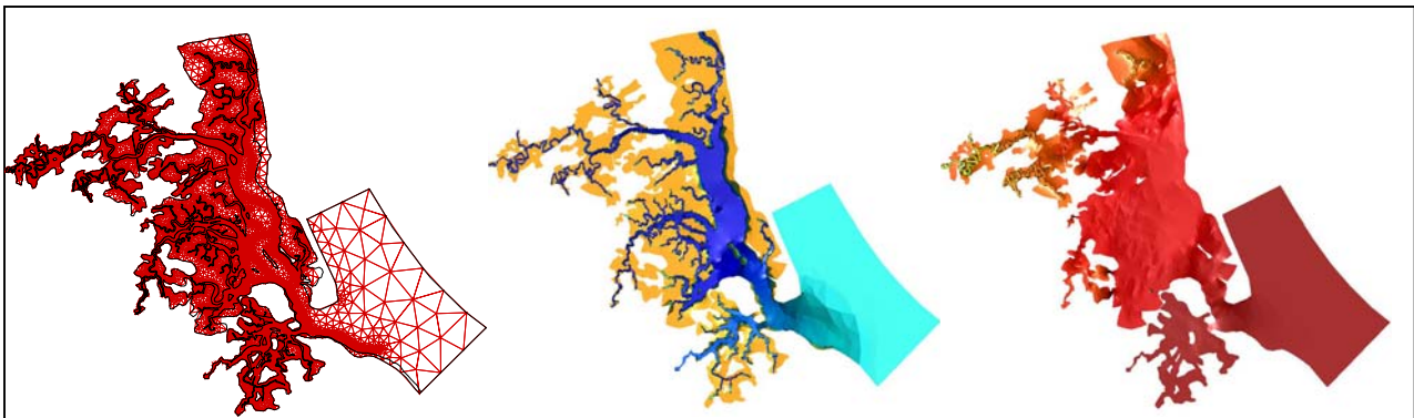
Fig 2.36. Creek resolving finite element grid (left) used in 2D PIE estuarine circulation-biogeochemistry model. Simulated water elevation at low tide (center) and high tide (right).
