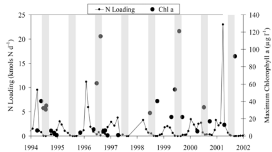
Fig 2.24. Relationship between N inputs from the watershed and Chl a concentrations in the Upper Parker River Estuary. The majority of the N inputs enter during the spring freshet while the major phytoplankton bloom occurs during summer (stippled line) when external inputs are low but water residence time is long. Our data suggests that internal recycling, driven in part by salinity changes, supports the mid-summer blooms.
