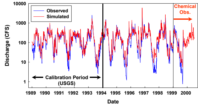
Fig 2.32. Observed (blue) and simulated (red) Ipswich River discharge. Model was calibrated using data from 1989 to 1994.
