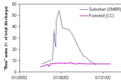
Fig 2.13. Fraction of total discharge that is composed of “new” water following a rain event in streams draining suburban and forested catchments, using silica and deuterium isotopes as tracers. New water is much more important in the suburban catchment, bypassing biogeochemically active subsystems.
