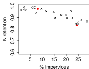
Fig 2.12. N retention (storage and/or denitrification) during 2001-2002 vs % impervious surface in headwater catchments. N export increases faster than N loading with imperviousness (Wollheim et al. submitted). Continued long term monitoring will allow us to determine year-to-year variability in retention and begin to understand the mechanisms whereby this high N retention occurs.
