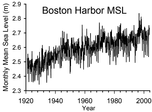
Fig 2.14 Monthly mean sea level (m) in Boston Harbor. MSL varies seasonally by about 20 cm due to changes in density (thermal effects). This seasonal cycle is highly variable owing to changes in climate and can have a large effect on the flooding frequency of salt marshes, which are situated at an elevation high in the intertidal zone.
