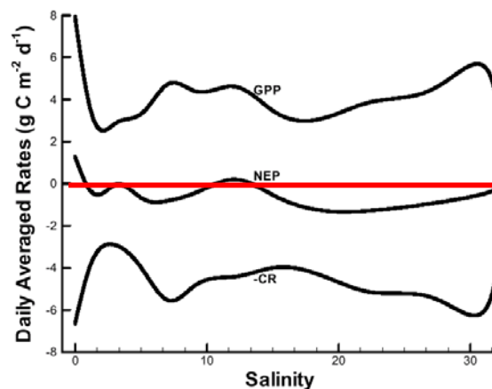
Fig 2.21. Depth integrated gross primary production (GPP), community respiration (-CR, plotted as negative value) and net ecosystem production (NEP) integrated over a 24 hr period as a function of salinity along estuarine axis. From Vallino and Hopkinson (submitted). NEP is positive in the oligohaline part of the estuary because of the diatom bloom, negative (heterotrophic) in most of the estuary, and approaches zero at the seaward end of the transect.
