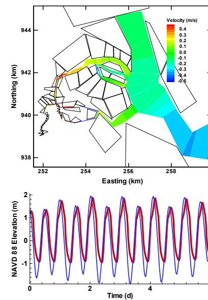
Fig 2.35. Instantaneous tidal velocities (Top) and tidal elevation at mouth and head of Rowley River (Bottom) from FEQ model. Non-filled polygons are marsh platforms.
